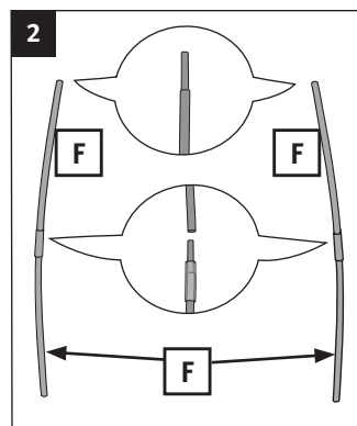
Connect two side poles [F] together for each side of the cab frame.
