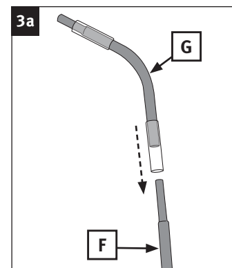
Insert the back hoop corner poles [G] over the end of the top back hoop side poles [F] set.
