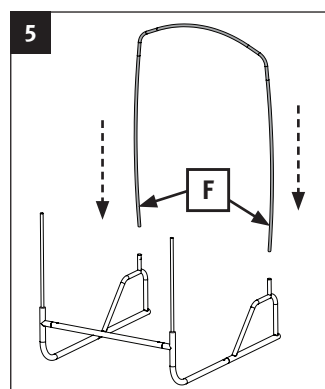
Insert the back hoop side pole assembly into the upper stub tubes on the right and left side of the frame.
